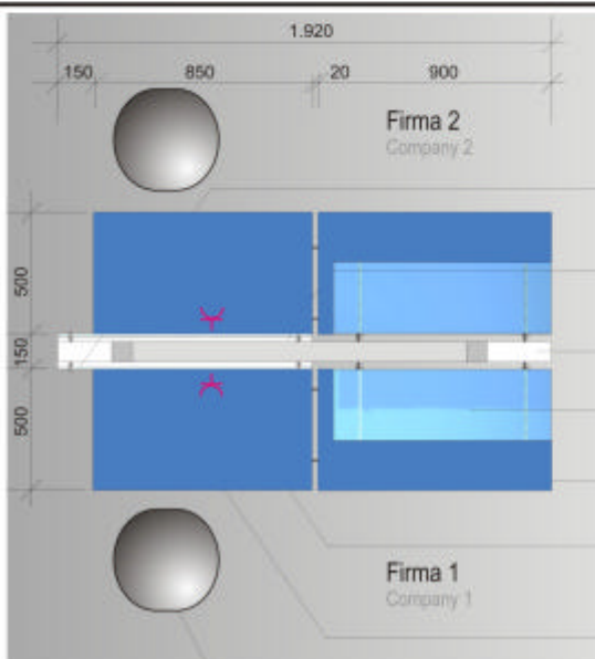
Grundriss Firmenstand Plan company stand
